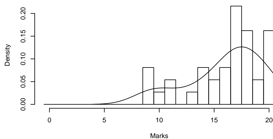
Practical assignment # of students 37, mean 16.05, median 17, stdev 3.34
