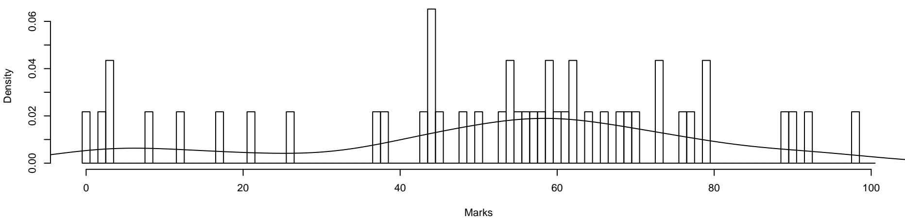
Total # of students 46, mean 52.13, median 56, stdev 25.38
